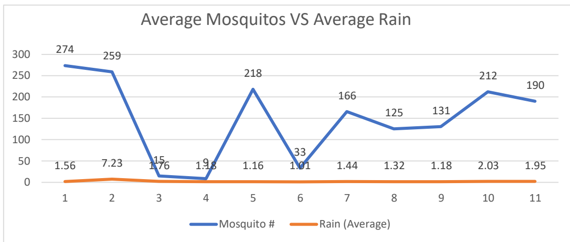
Figure 1 October trap counts vs rain
